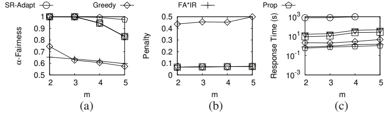
Fig. 10: Effect of m on Anti-correlated
