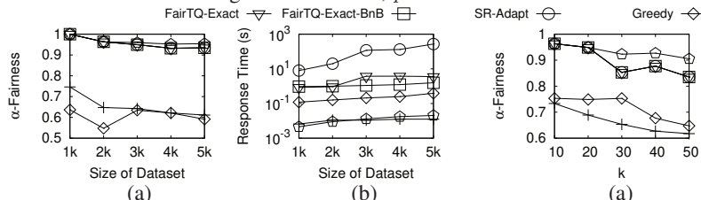
Fig. 6: Effect of |D| on COMPAS
