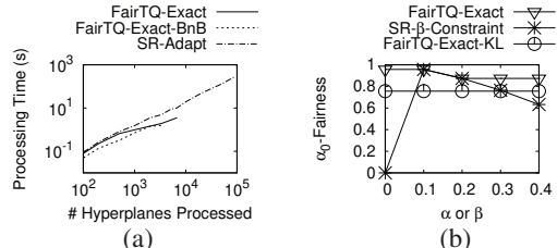
Fig. 5: # Hyperplanes & Fairness on COMPAS
