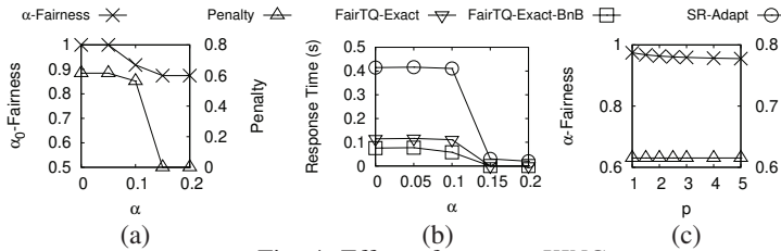
Fig. 4: Effect of \alpha , p on XING
