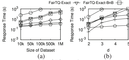
Fig. 9: Effect of |D| and d on Independent
