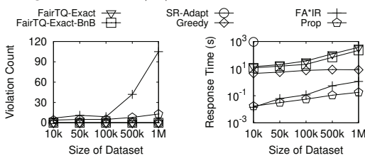
Fig. 8: Effect of |D| on DOT
